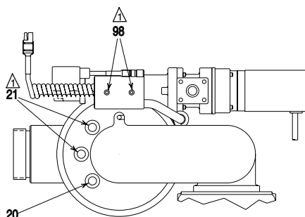
VIEW E-E
