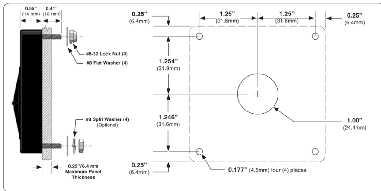
Figure 3-4: Smart-Switch Controller Panel Cutout
