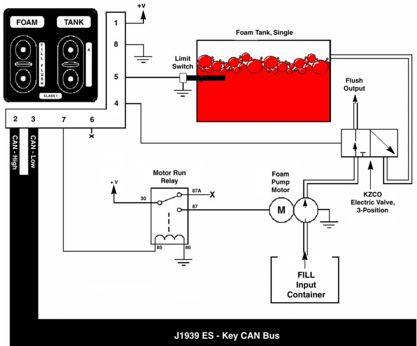
Figure 6-1: Typical Single Tank Electrical Schematic Overview
