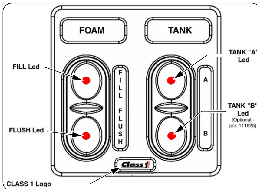
Figure 8-1: Smart-Switch Troubleshooting LEDs
