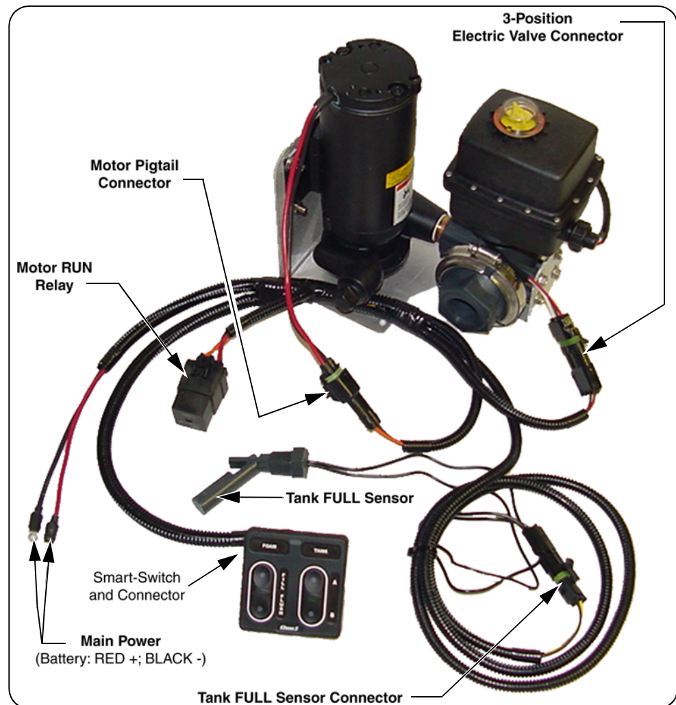
Figure 3-5: Interconnecting Harness, Single Tank
