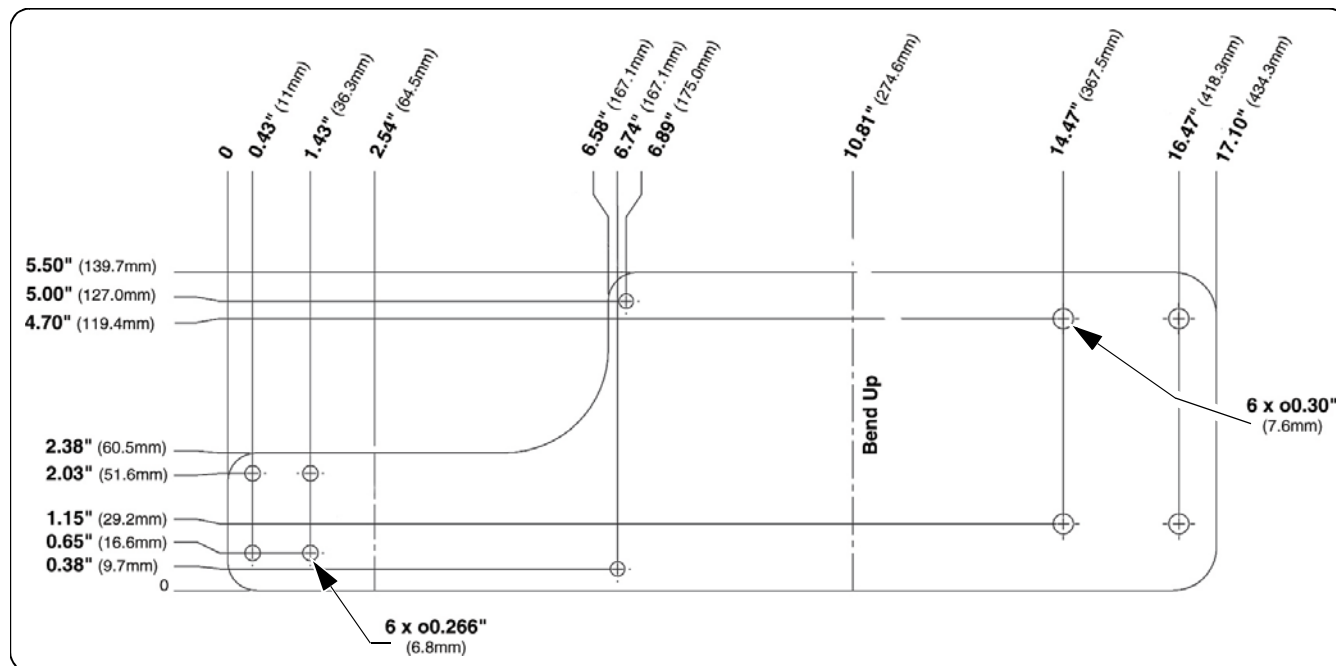
Figure 3-2: Mounting Bracket Layout
