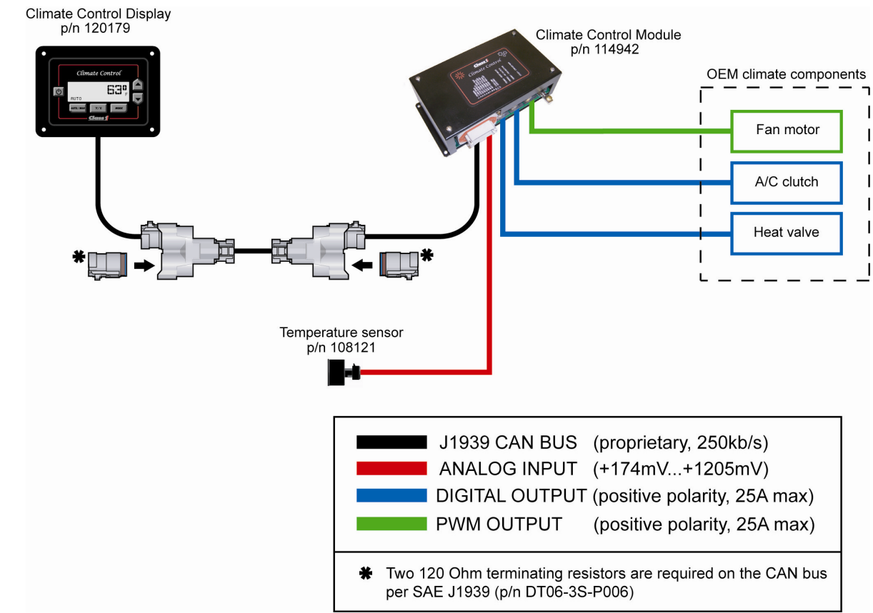
Figure 2. Typical climate control system layout
