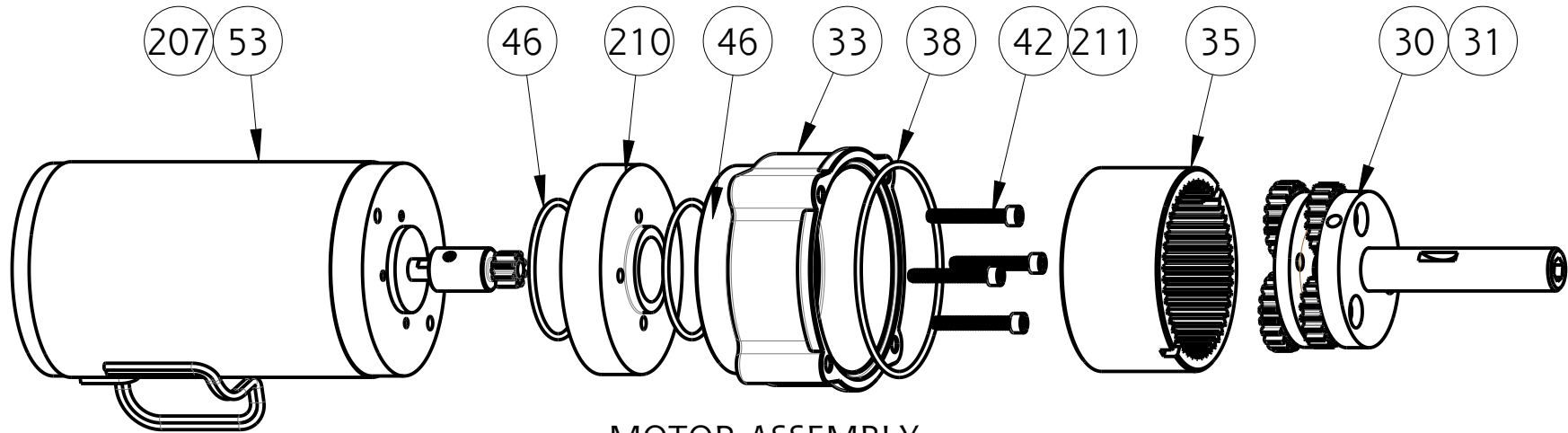
MOTOR ASSEMBLY
