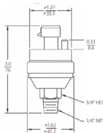
93000060 – Pressure Sensor with Connector (NEW)
