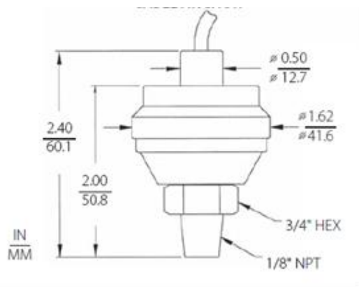
93000050- Pressure Sensor with Cable (OLD)
