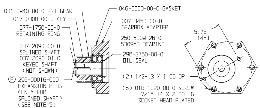
DRIVE ASSEMBLY COMPONENTS
