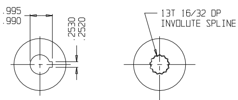
DRIVE SHAFT DETAIL (SCALE 2:1)
